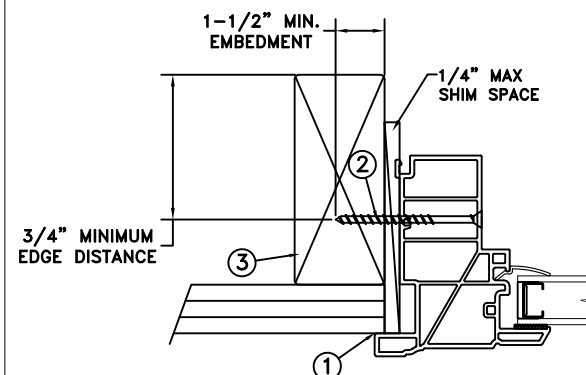
FRAME JAMB SECTION (TYP) HORIZONTAL SECTION
